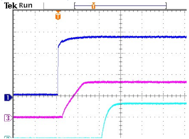
Figure 14: Control turn on at 12Vin, 3.3V /20A Ch1: Enable, Ch3: Vo, Ch2: PG
