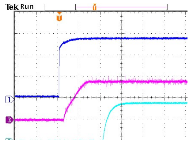
Figure 18: Control turn on at 12Vin, 0.9V /20A Ch1: Enable, Ch3: Vo, Ch2: PG
