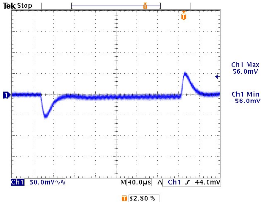
Figure 21: Transient response, 2.5V /20A, Ch1: Vo
