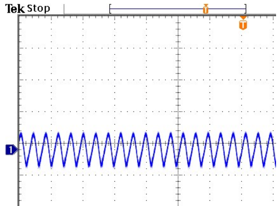
Figure 10: Output ripple & noise at 12Vin, 1.5V/20A out
