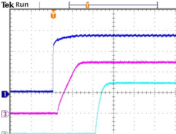
Figure 13: Control turn on at 12Vin, 5.0V /20A Ch1: Enable, Ch3: Vo, Ch2: PG
