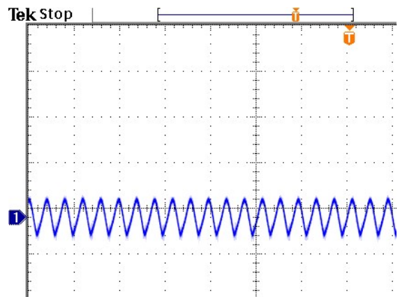
Figure 12: Output ripple & noise at 12Vin, 0.9V/20A out
