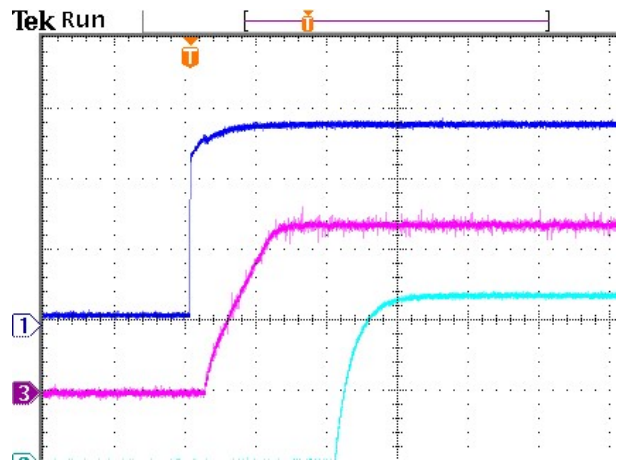
Figure 17: Control turn on at 12Vin, 1.2V /20A Ch1: Enable, Ch3: Vo, Ch2: PG
