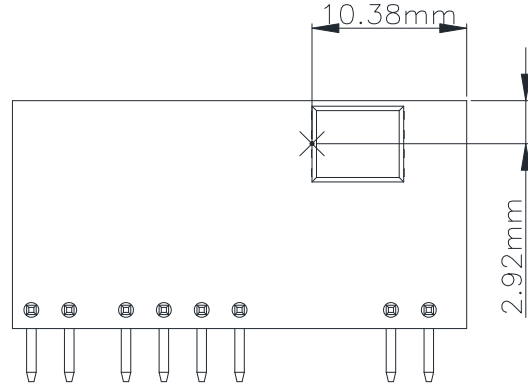
Figure 28: Temperature measurement location* The allowed maximum hot spot temperature is defined at 125°C
