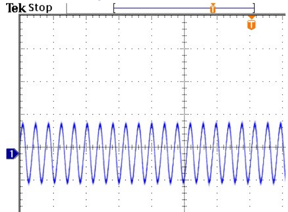
Figure 8: Output ripple & noise at 12Vin, 3.3V/20A out
