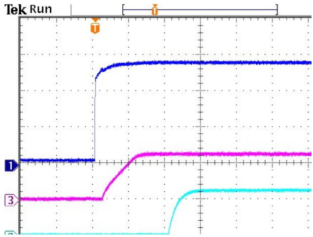
Figure 15: Control turn on at 12Vin, 2.5V /20A Ch1: Enable, Ch3: Vo, Ch2: PG
