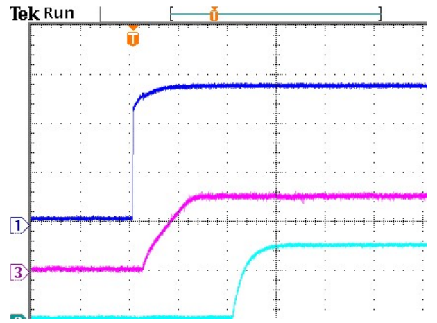
Figure 16: Control turn on at 12Vin, 1.5V /20A Ch1: Enable, Ch3: Vo, Ch2: PG
