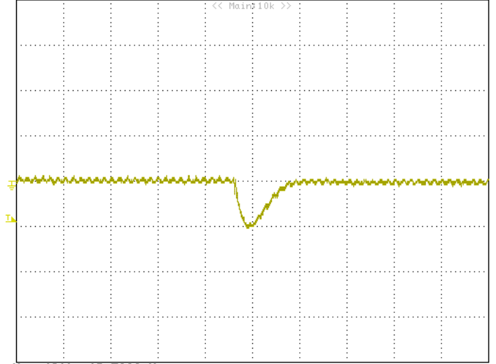
Figure 20: Typical transient response to step load change at 2.5A/\mu S from 50% to 100% of I_o , max at 5V_{in} , 3.3V_{out} ( C_{out} = 1\mu F ceramic, 10\mu F tantalum) ( 100mV/div , 10\mu S/div )
