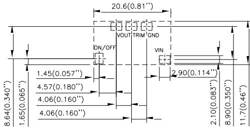
RECOMMAND PWB PAD LAYOUT
