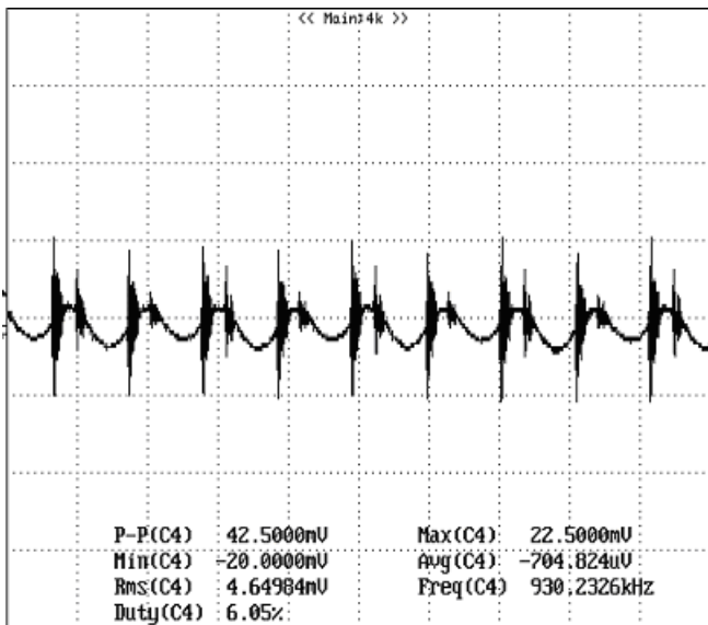
Figure 15: Output voltage ripple at nominal input voltage and rated load current ( I_o=10A ) (20 mV/div, 2us/div) Load capacitance: 1\mu F ceramic capacitor and 10\mu F tantalum capacitor. Bandwidth: 20 MHz. Scope measurements should be made using a BNC cable (length shorter than 20 inches). Position the load between 51 mm to 76 mm (2 inches to 3 inches) from the module.
