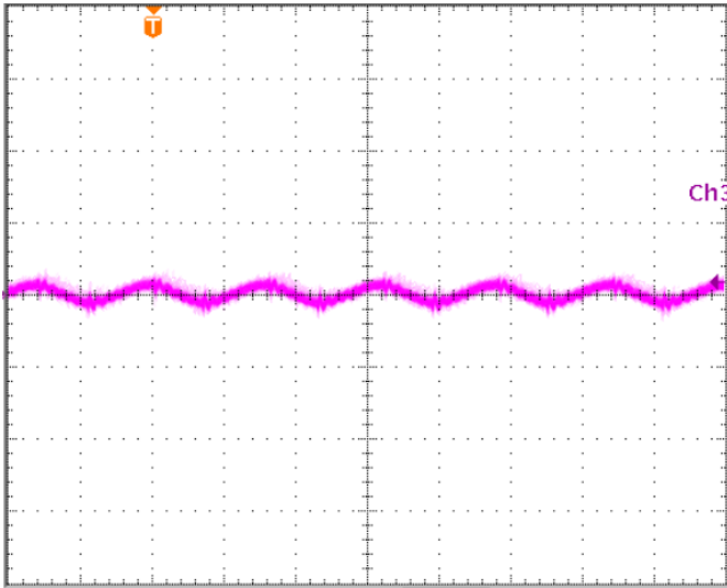
Figure 12: Input reflected ripple current, i_s , through a 12\mu\text{H} source inductor at nominal input voltage and max load current ( 25\text{mA}/\text{div} , 2\mu\text{s}/\text{div} ).
