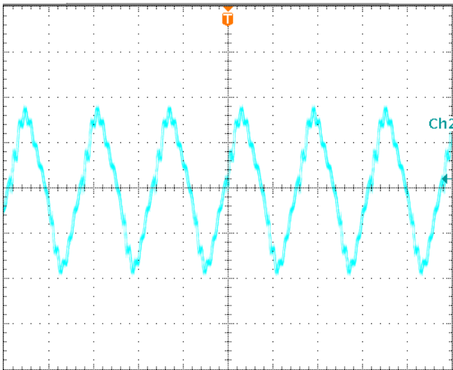
Figure 14: Output voltage ripple at nominal input voltage and max load current ( 30\text{mV}/\text{div} , 2\mu\text{s}/\text{div} ) Load capacitance: 1\mu\text{F} ceramic capacitor and 10\mu\text{F} tantalum capacitor. Bandwidth: 20\text{MHz} .
